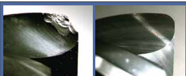
This end mill arrived with heavy chipping on the flute end (left). Guhring Reconditioning restored a correct cutting edge (right). The result: Greatly extended tool life and significant cost savings.
